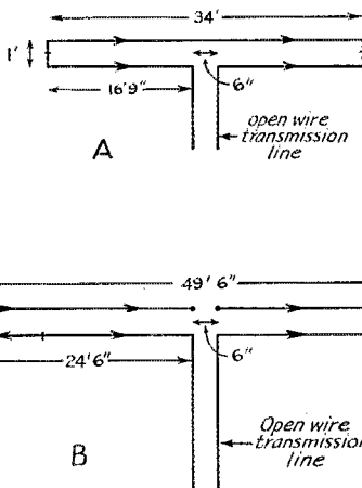
Fig. 3 — The 2-wire half-wave antenna (A) and the 2-wire three-quarter wave antenna (B). Dimensions are given for the 14- to 14.4-Mc. band.
