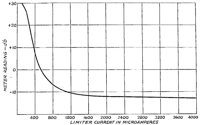
Fig. 4 — Noise in a.f. output of the receiver as a function of carrier strength, measured by rectified grid current in the limiter.
