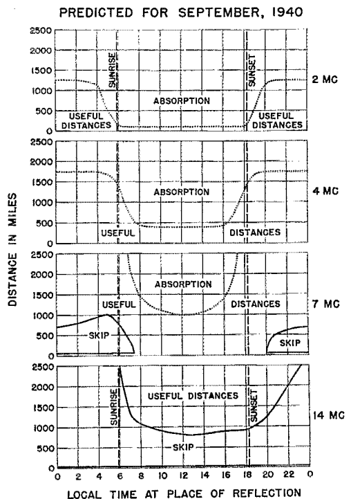
Fig. 2 — Useful distances for radio wave propagation via the regular layers of the ionosphere, predicted for September, 1940. The 28-Mc. and 56-Mc. bands will be useful only for local transmissions (optical and quasi-optical paths).
